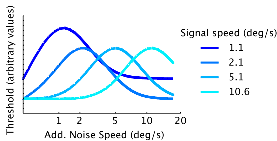
Fig. 4. Model results, simulating the experimental conditions. The different curves show the different signal speed conditions. The model shows clear resemblance to the experimental data (see Fig. 2b). Notably, it shows a lawful shift in the position of the top of each curve towards higher noise speeds for higher signal speeds. Moreover, the results also show an increased offset for low signal speed conditions, and a constant width of the different curves.
