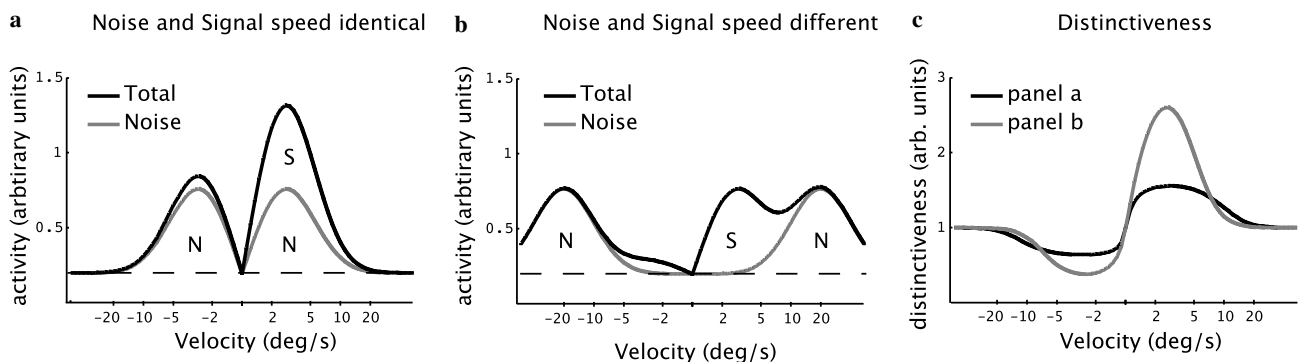
Fig. 5. Explanation of the increased thresholds when signal and noise speeds are similar compared to conditions where they differ. (a) A condition where noise and signal speed are identical. Shown are, the total activity ( T ) and the part of it that is caused by noise dots ( N ) and signal ( S ) dots. The figure is a slice through Fig. 3d, slicing through the origin and the maximum; negative and positive velocities in this graph represent therefore motions in opposite directions (the absolute value of the x -axis being the speed of the motion). The horizontal dashed line represents the baseline ( b ) in the model. (b) As in (a), but now for a condition in which signal and noise speeds differ. By comparing (a and b), one can see that the signal ( S ) constitutes a large part of the total activity over a wide range of velocities in (b) (from about 1 to 5 deg/s), whereas in (a) it is always accompanied by an increase in noise (in both “positive” and “negative” directions). Comparing the activities in opposite directions, as is done when calculating the distinctiveness measure (c), it is clear that the relative contribution of signal ( S ) is lower in the case when signal and noise speeds are identical, compared to when they differ. Therefore the final threshold (the inverse of the distinctiveness) will be higher for low-speed conditions of the noise.
