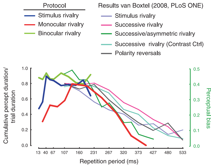
Figure 6. The temporal limits in terms of pattern repetition periods for binocular rivalry, stimulus rivalry, and monocular rivalry. The fat lines are data obtained in Experiment 4 . The thin lines are data obtained in a previous study (van Boxtel, Alais, Erkelens et al., 2008 ). The average of the cumulative percept duration over subjects is plotted. The data show that the monocular rivalry data fall within the normal spread of the data obtained with other protocols. An explanation of conditions can be found in van Boxtel, Alais, Erkelens et al. ( 2008 ). Briefly, successive rivalry is induced when the intermittently shown stimuli are presented in temporal anti-phase (such as in binocular rivalry conditions, Experiment 2 ). Successive/asymmetric conditions are similar to successive rivalry, but the temporal phase difference is <180 degrees. In these experiments subjects either perceived binocular rivalry or repetitive dichoptic masking (van Boxtel, Alais, Erkelens et al., 2008 ). Therefore, we used the perceptual bias as a measure (y-axis on the right), which shows the transition from binocular rivalry to dichoptic masking. In the polarity reversal experiments both patterns reversed in contrast polarity at each presentation.
